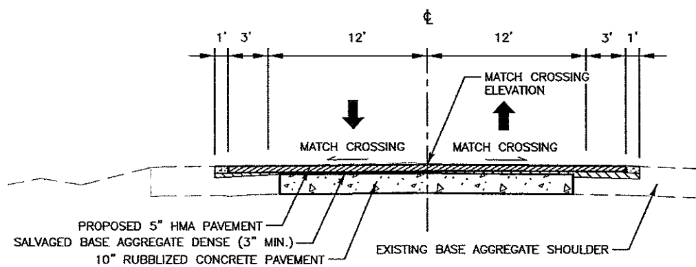
TYPICAL FINISHED SECTION AT RAILROAD CROSSING
