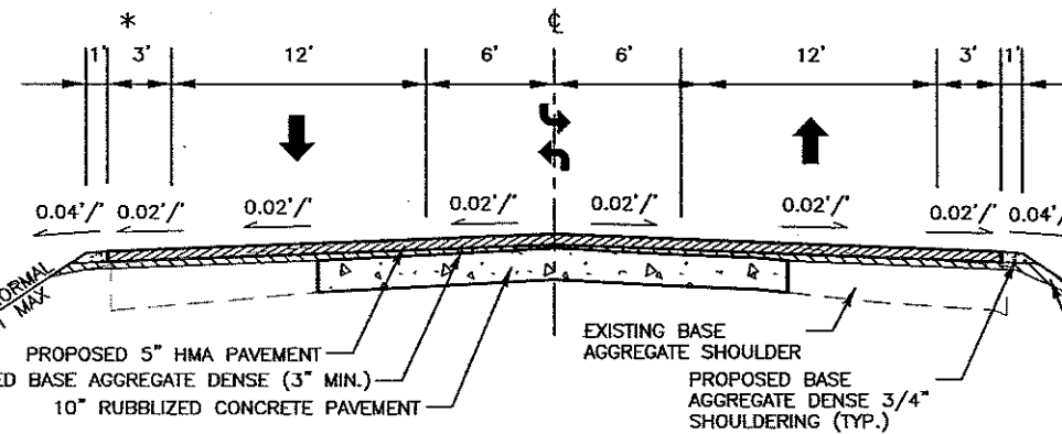
TYPICAL FINISHED SECTION
