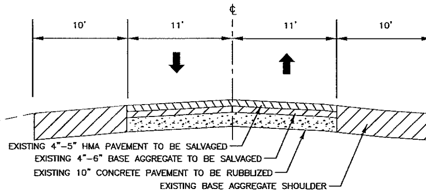
TYPICAL EXISTING SECTION
