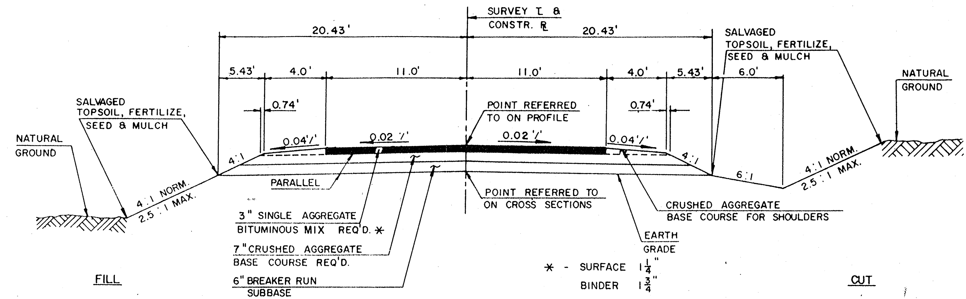
TYPICAL SECTION FOR C.T.H. "U" ( FOR INFORMATIONAL PURPOSES ONLY ) ( NOT PART OF THIS CONTRACT )
