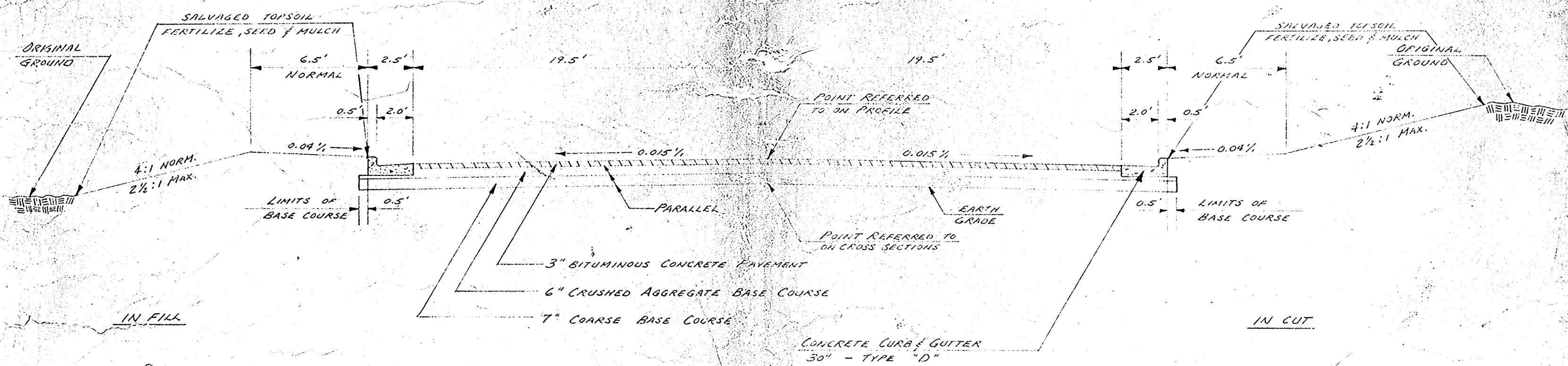
TYPICAL URBAN SECTION TWO MILE ROAD STA. 41+50 - STA. 53+50
