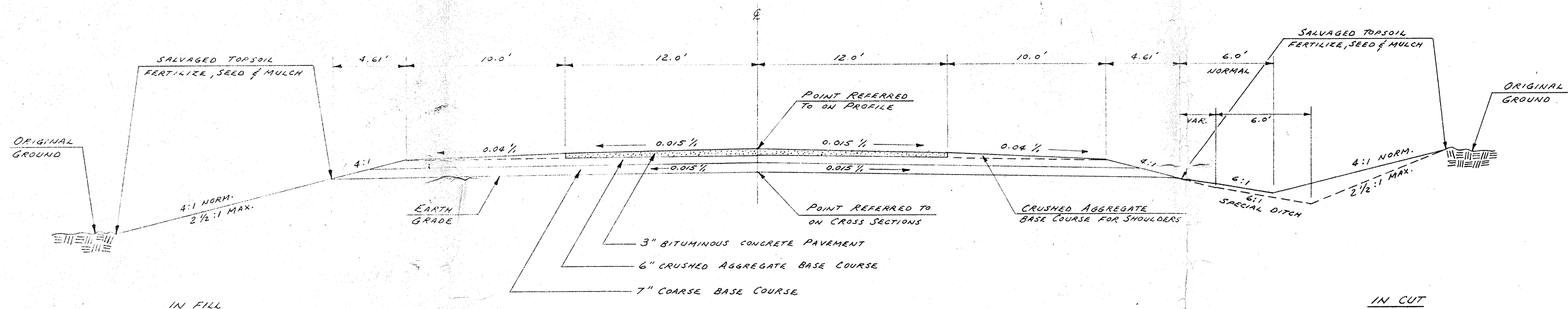
TYPICAL FINISHED SECTION C.T.H. "CA"
