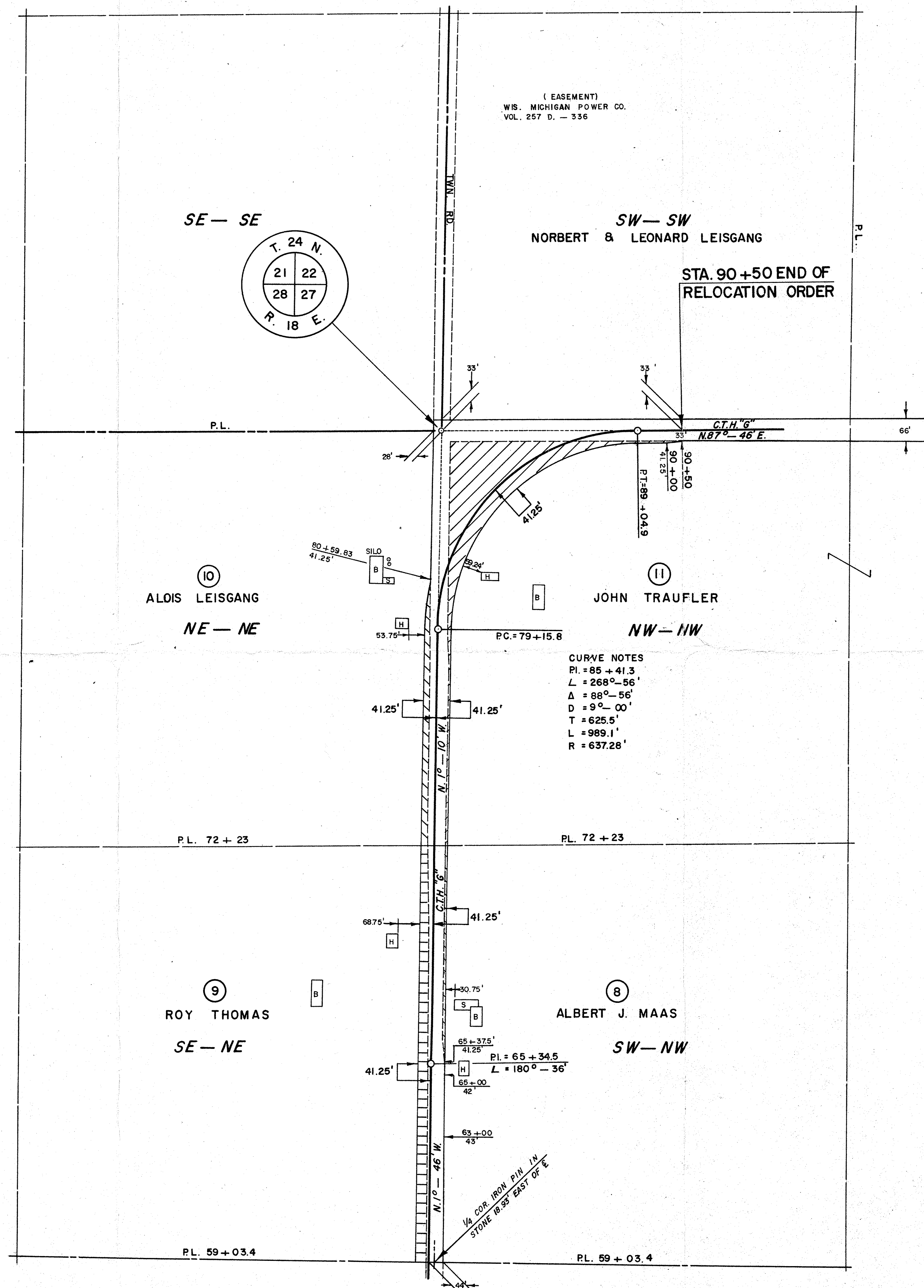
NO. OWNER ACRES REQ'D. RODS OF FENCING INTEREST REQUIRED TO MOVE TO BUILD ✓ 8 ALBERT J. MAAS DOLORES ZEHREN 0.06 42 HIGHWAY EASEMENT ✓ 9 ROY THOMAS 0.92 76 " " ✓ 10 ALOIS LEISGANG 0.35 40 " " ✓ 11 JOHN TRAUFLER 2.07 103 FEE SIMPLE
